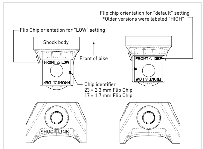
Figure 2 - Flip Chip Orientation
