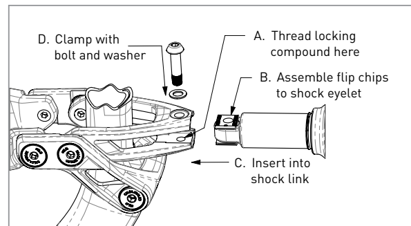
Figure 3 - Assembly Procedure
