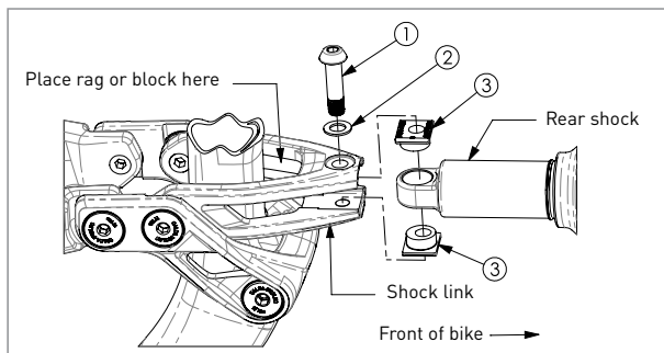
Figure 1 - Exploded View
