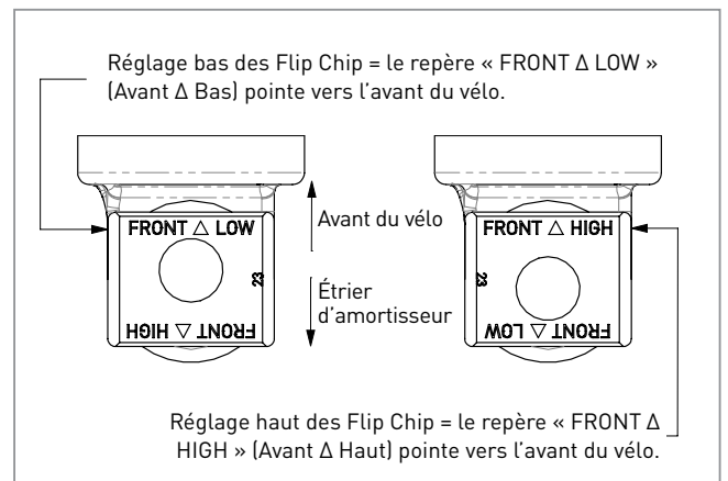
Figure 2 - Orientation des Flip Chip
