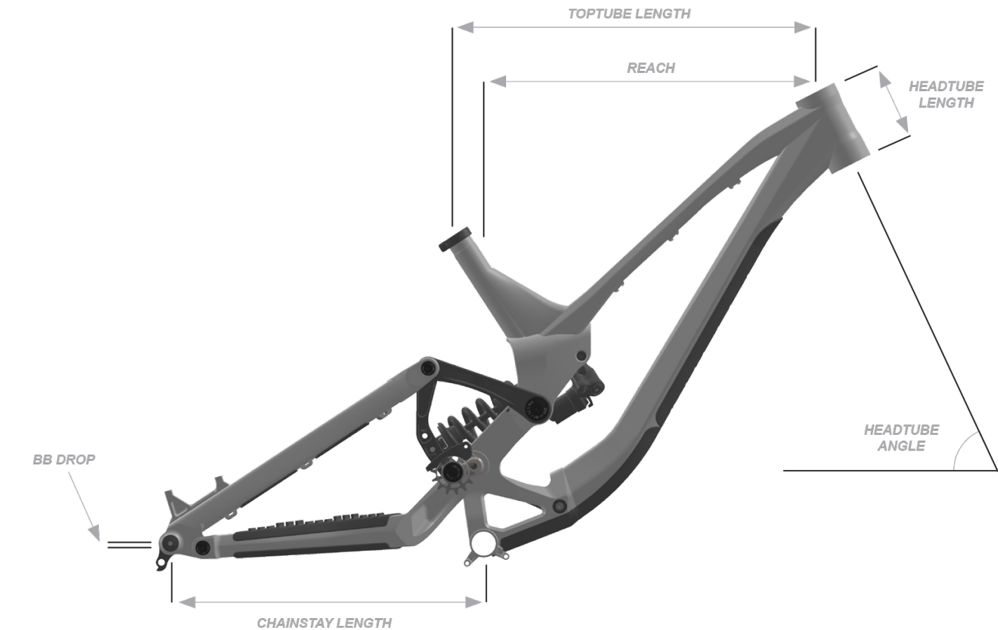
2027 Intense M1 Frameset Geometry & Size Chart
