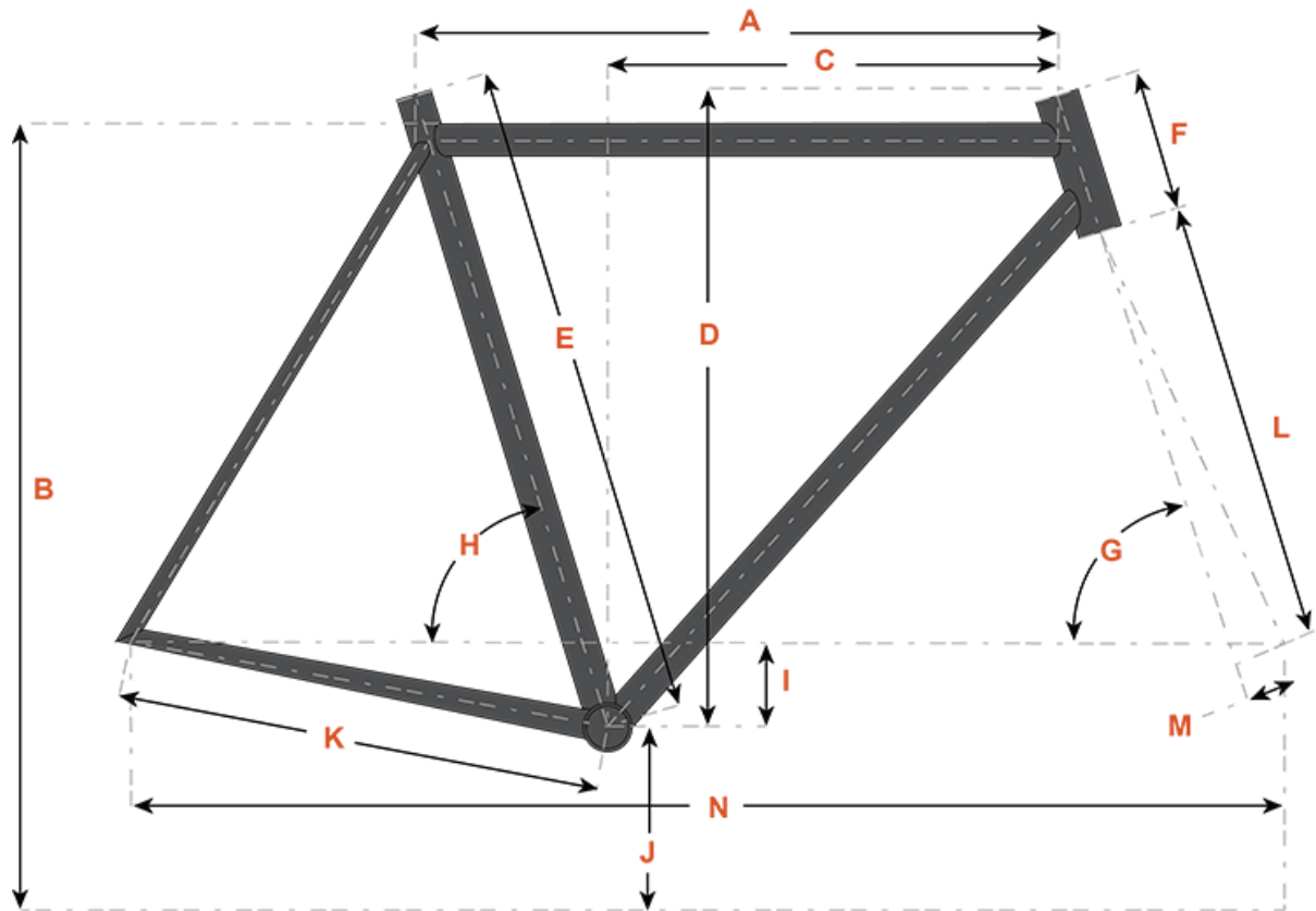
2027 Salsa Tributary Apex Eagle SUS 29 - Charcoal Geometry Table
