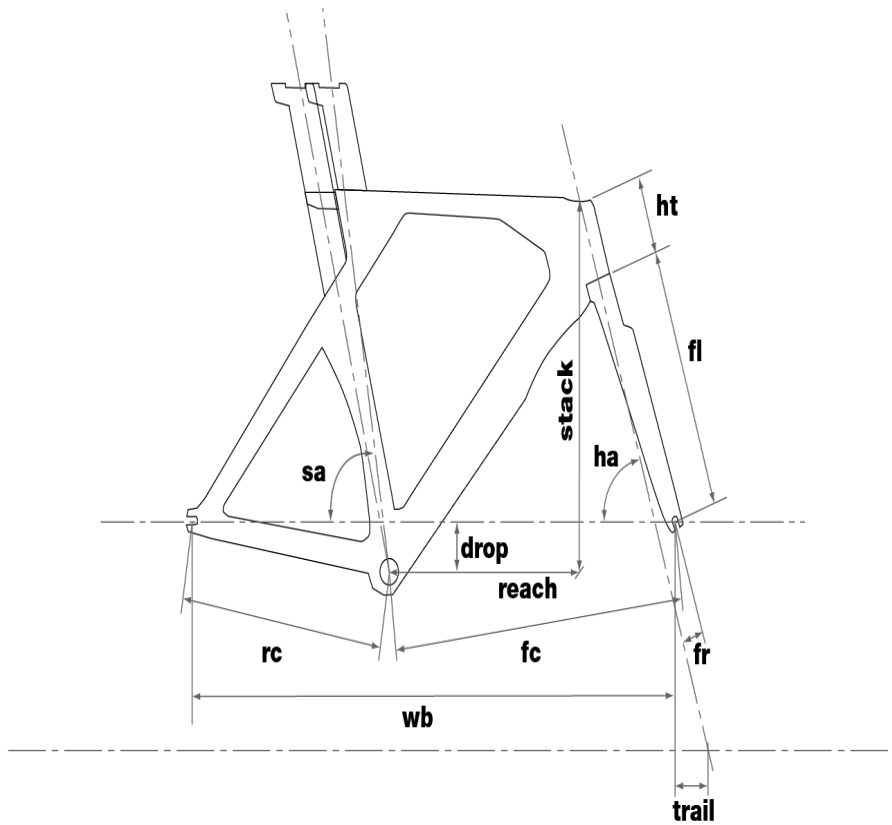
2022 BMC TIMEMACHINE Geometry Chart
