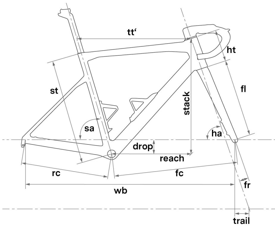
BMC Teammachine SLR01 THREE Road Bike Geometry Chart
