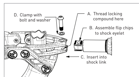
Figure 3 - Assembly Procedure
