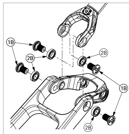
Link Bolts Detail - Rustler
