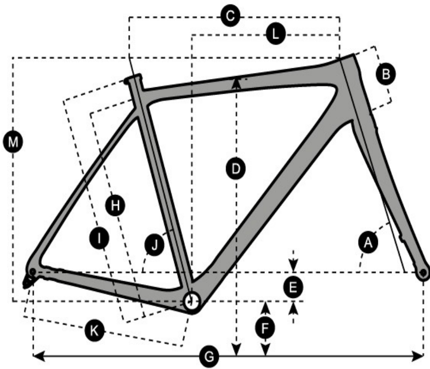
SCOTT METRIX 30 EQ BIKE Geometry Chart (INCHES)
