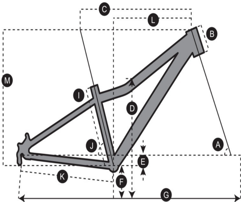
SCOTT SCALE 24 DISC YELLOW BIKE Geometry Chart (INCHES)
