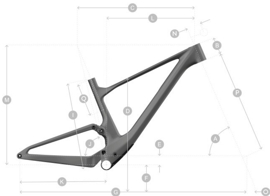
SCOTT SPARK RC PRO BIKE Geometry Chart (INCHES)
